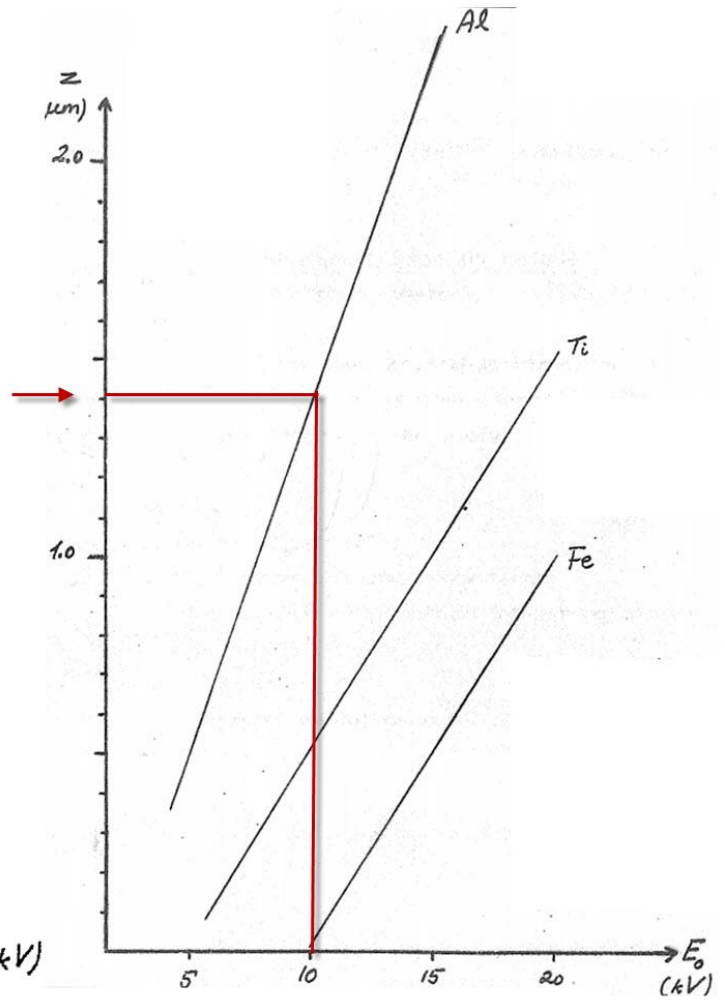
Emission depth of K characteristic x-ray
