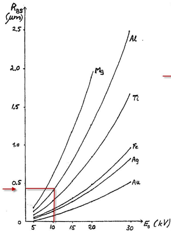
Emission depth of BSE
