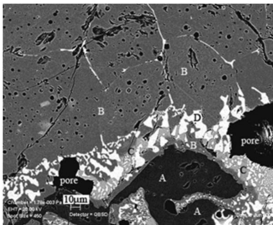
Fig. 4. Backscattered electron scanning electron microscopy image in region I, showing the CT-rich grain boundaries on the MT side of the joint. The eutectic phase of MT2–CT, large M2T clusters (A), and the individual phases of MT (B), M2T (light gray, C) and CT (white, D), as well as the pores and cracks (black) can be observed.
