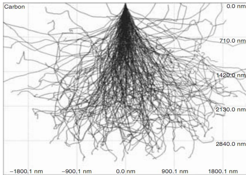
Carbon Z = 12
