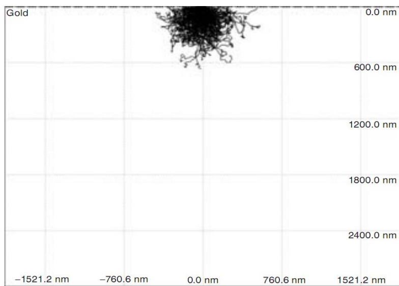
Gold Z = 79
