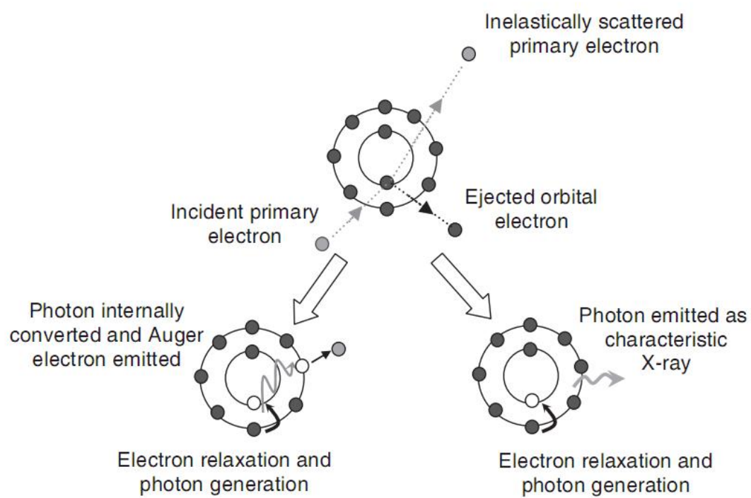
Schematic illustration of the process of inner electron ionisation and the production of either a characteristic X-ray or Auger electron
