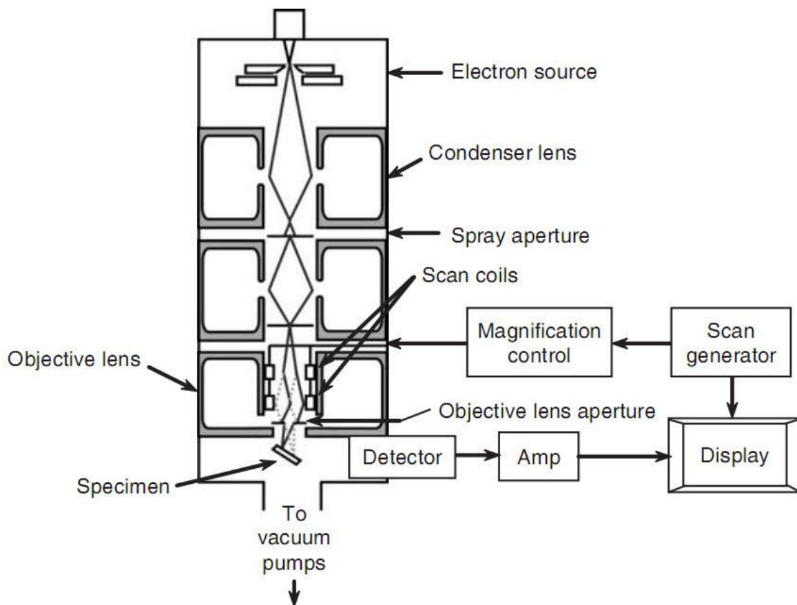
Simplified schematic diagram of the basic components of an SEM.
