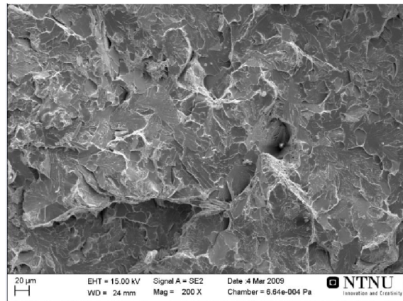
Brittle, Cleavage Fracture / Kløvningsbrudd
