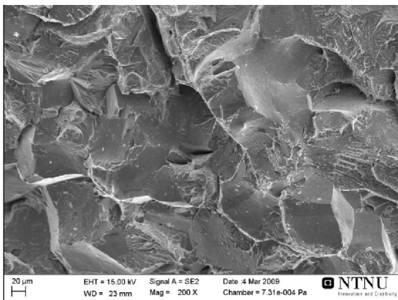
Intergranular Fracture / Interkrystallinsk Brudd
