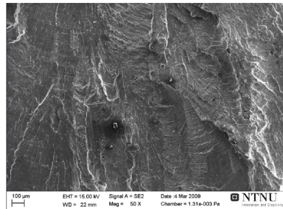
Fatigue fracture / Utmattingsbrudd
